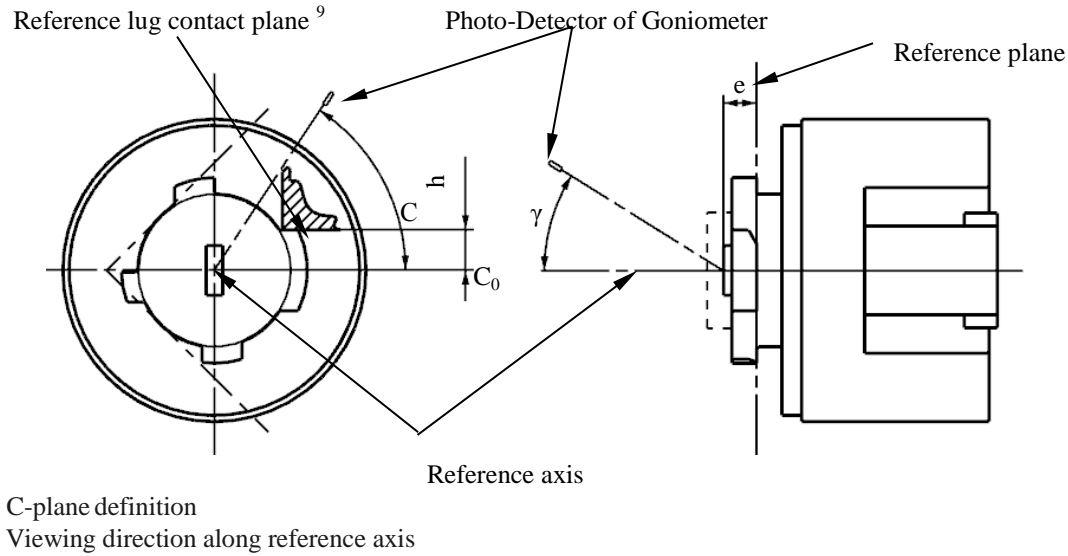
Figure 5 Set-up to measure the luminous intensity distribution for L1B
