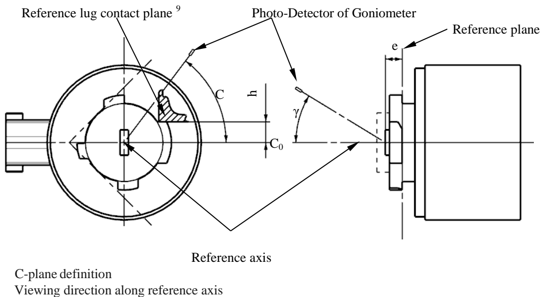
Figure 4 Set-up to measure the luminous intensity distribution for L1A
